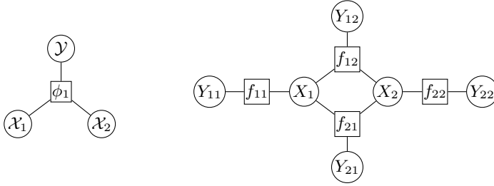
Figure 5. The par-factor graph (left) and instantiated factor graph (right) of Example 3.
