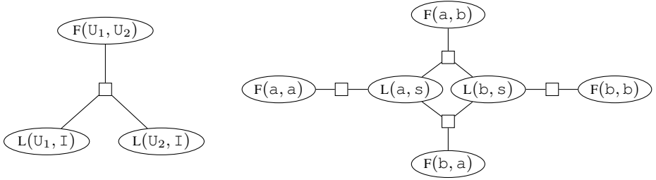
Figure 7. The par-factor graph representing Formula (13) (left) and an instantiated factor graph based on the sets \mathbf{U} = \{\text{alice}, \text{bob}\} and \mathbf{I} = \{\text{starwars}\} (right). For readability, we used F for FRIENDS, L for LIKES, a for alice, b for bob, and s for startrek.
