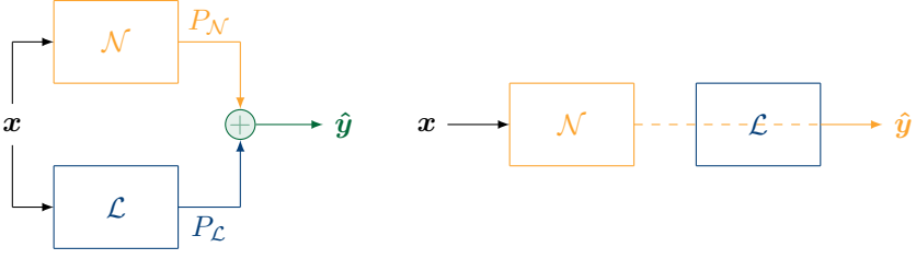
Figure 11. Abstract representation of parallel (left) and stratified (right) architectures. Symbol \oplus denotes that the output \hat{y} is computed by “composing” the neural predictions with the logical predictions.
