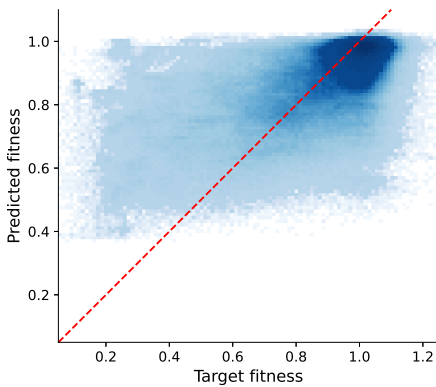
(c) Double deletion with semantic loss, R^2 = 0.377 .
