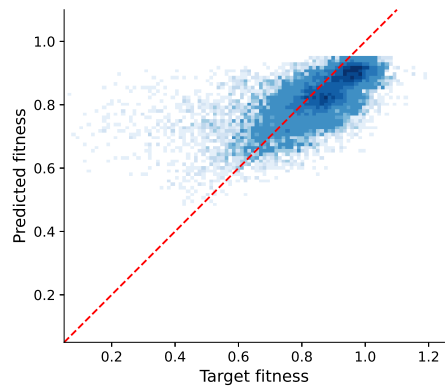
(d) Triple deletion with semantic loss, R^2 = 0.415 .
