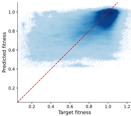
(a) Double deletion, R^2 = 0.360 .
