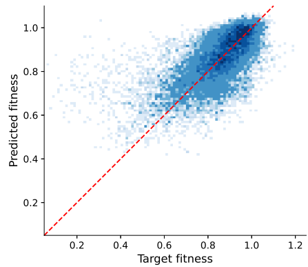
(b) Triple deletion, R^2 = 0.380 .
