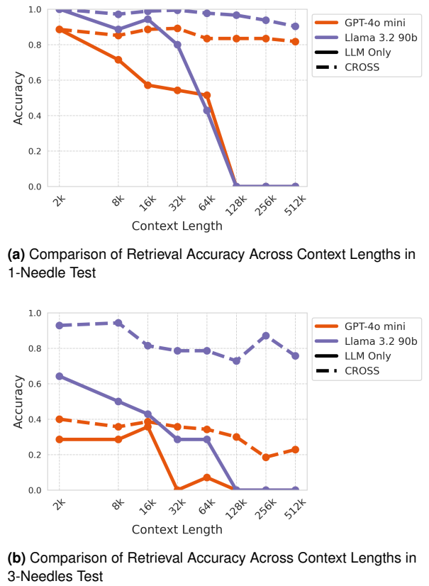
Figure 2. Retrieval Accuracy Across Different Context Lengths
