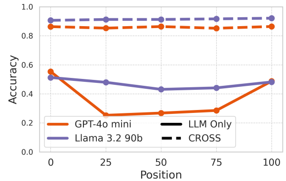
Figure 3. Retrieval Accuracy Comparison Across Needle Positions
