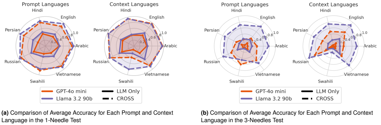
Figure 1. Radar Plots Comparing Average Accuracy in Different Tests
