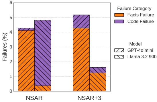
Figure 17. Error sources under NSAR and NSAR+3 .
