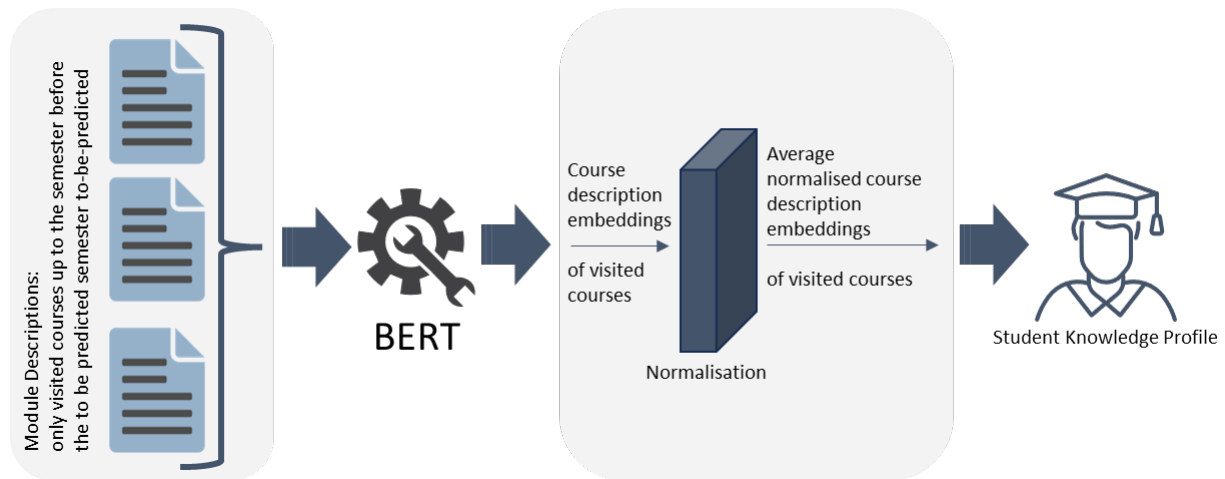
Fig. 2. Calculating students knowledge profile
